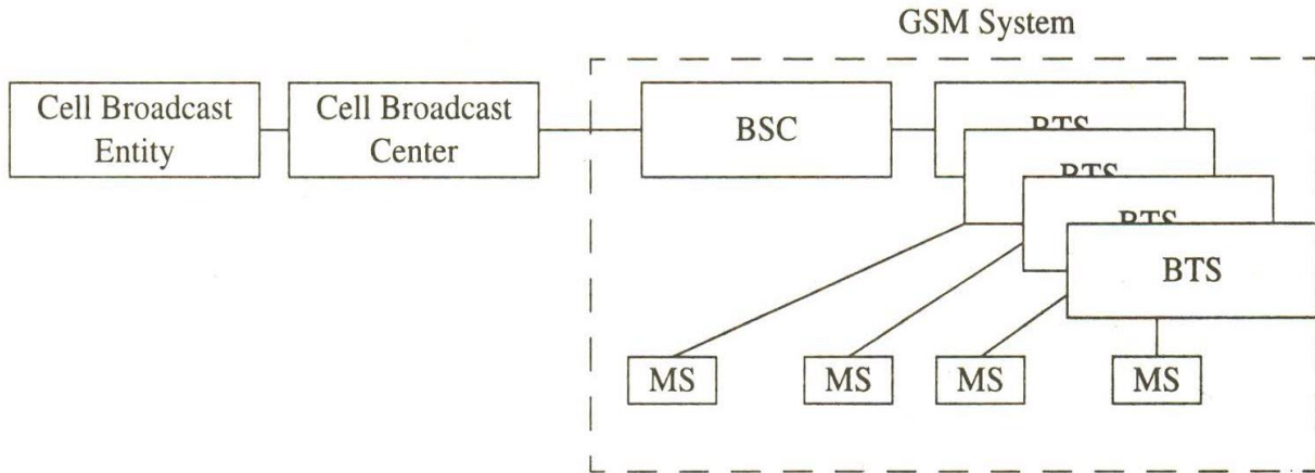
Fig. 10.11 Architecture of SMSCB
