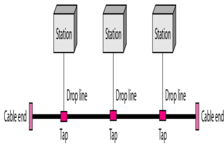
Bus Topology
