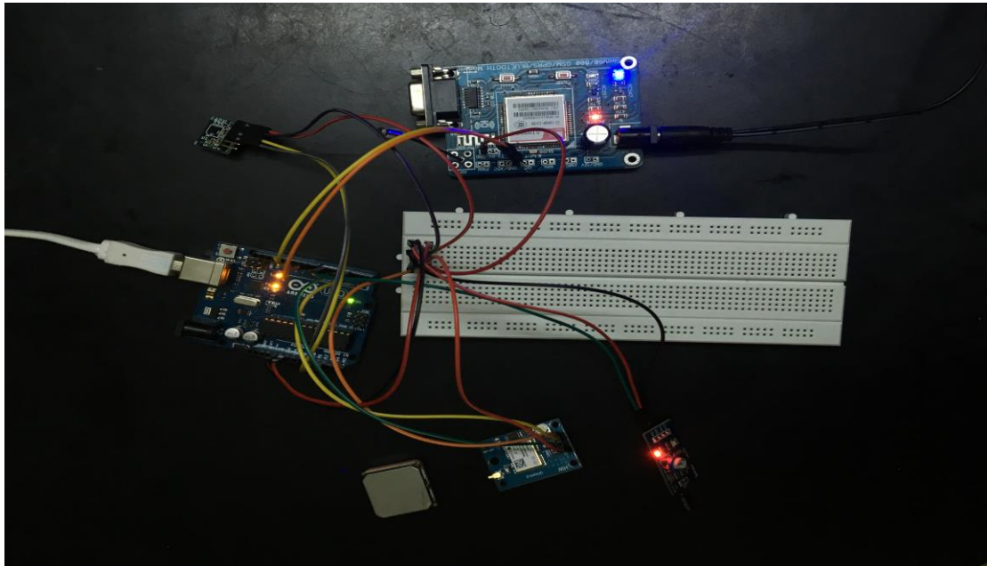
Fig 11: interfacing controller with all other module
