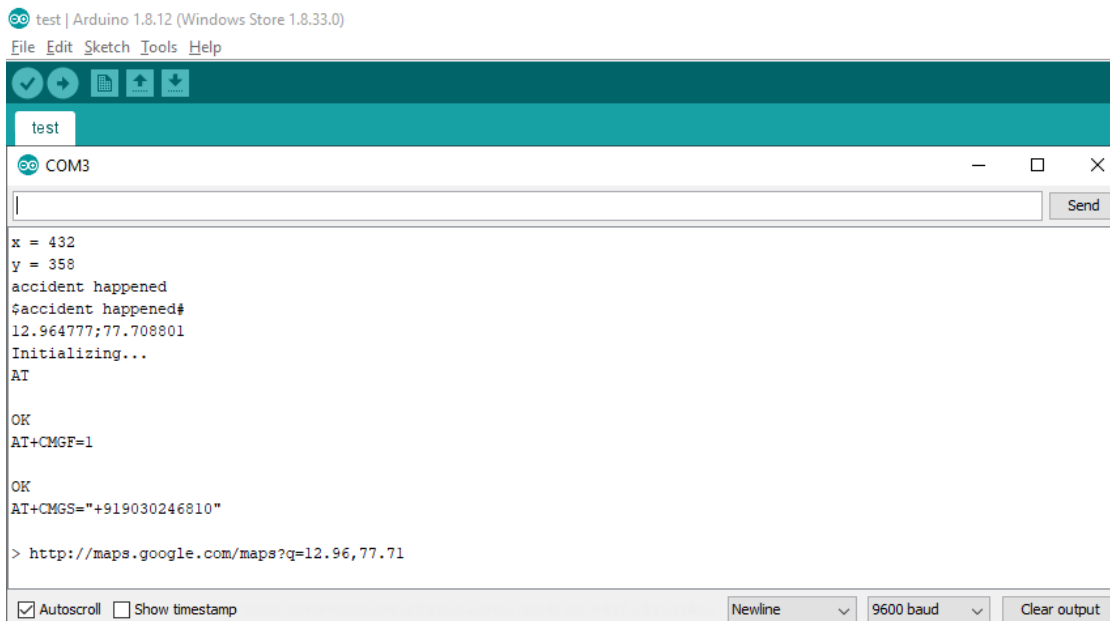
Fig 16: Testing of accident detection
