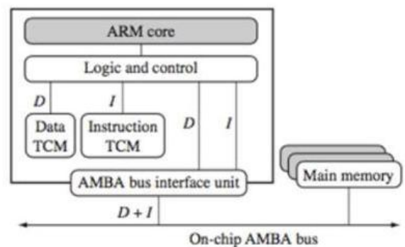
A simplified Harvard architecture with TCMs.
